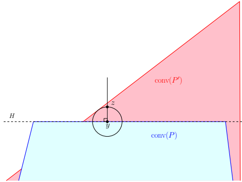
Figure 1: Lemma 2.2: \partial\text{conv}(P) and \partial\text{conv}(P') must be close.
