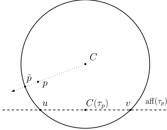
Figure 4: Diagram for Lemma A.3.
